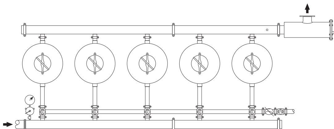
Array of gravel/sand filters with a single control filter
