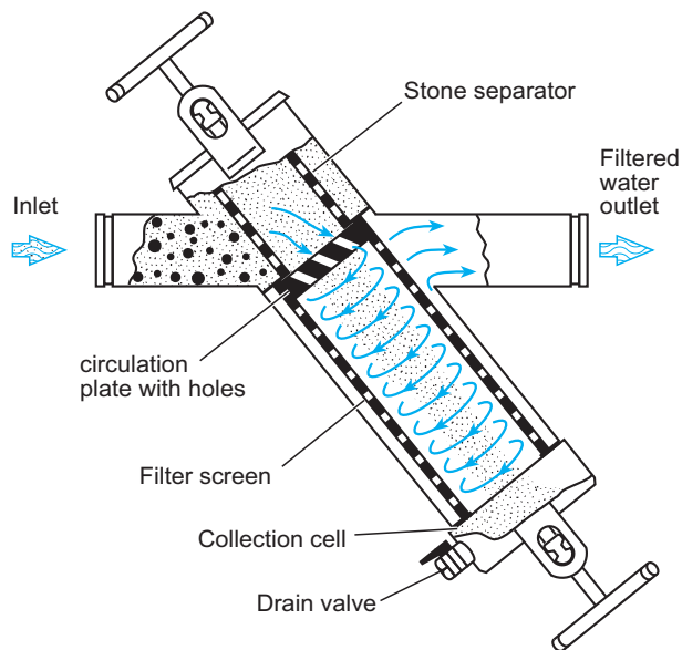
AUTOMATIC WATER CIRCULATING FILTER WITH STONE SEPARATOR SCHEMATIC DRAWING
